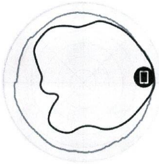
Figure 3. 5GHz Azimuth Antenna Patterns
