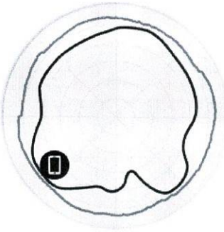
Figure 2. 2.4GHz Azimuth Antenna Patterns
