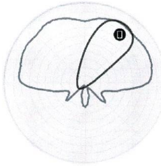
Figure 5. 5GHz Elevation Antenna Patterns
